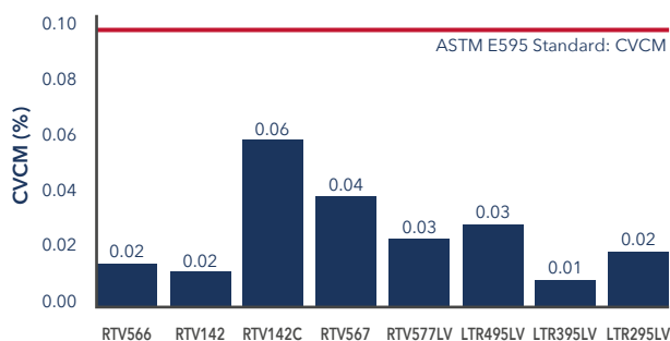
ASTM E595 Results: CVCVM (≤0.10%)
